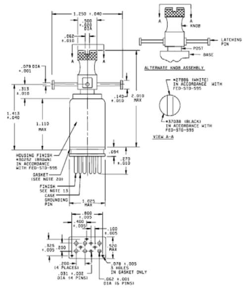
Mount 09 & Terminals GG: Track Mount, Gold Plated Plug In
