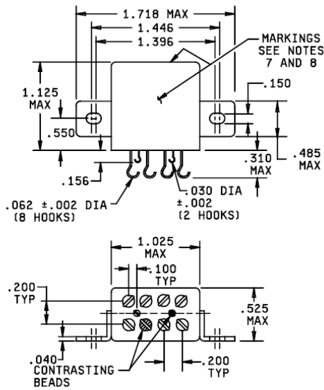
Mount 08 & Terminals AT: Horizontal Flange Mount, Tin Plated Solder Hooks
