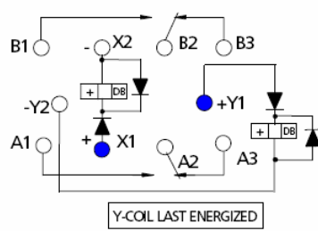
ELS210 OPTIONAL INTERNAL VOLTAGE SUPPRESSOR (-5 VDC MAX.)
