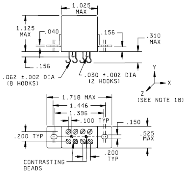
Mount 03, Terminals AT: Raised Vertical Flange Mount, Tin Plated Solder Hooks
