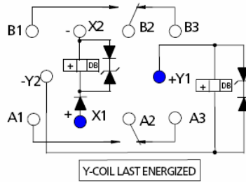
ELS210 Track Mount OPTIONAL INTERNAL VOLTAGE SUPPRESSOR (-42 Vdc MAX.)
