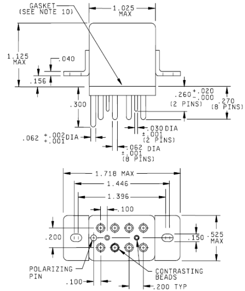
Mount 03, Terminals CG: Raised Vertical Flange Mount, Gold Plated Plug In
