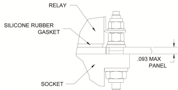
MOUNTING DETAIL 3 PLACES
