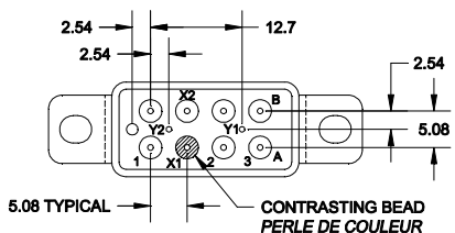
DETAIL VIEW A
