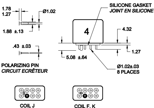
GOLD PLATED SORTIES DOREES
