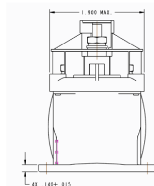
SM15WA1 height *other dimensions same as below
