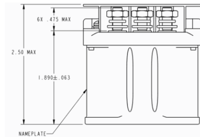
SM15WA1 height *other dimensions same as below
