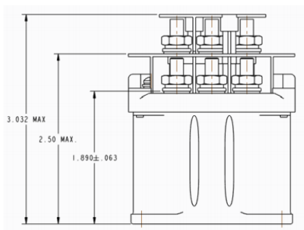
SM15CWD8, SM15CXD24, SM15CXA11, SM15CWD9 DIMENSIONS
